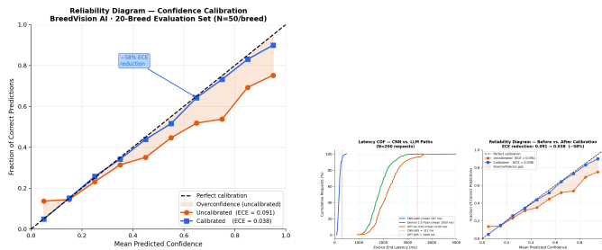
(a) Reliability diagram: uncalibrated (ECE=0.091) vs. calibrated (ECE=0.038). Shaded area = overconfidence gap.
